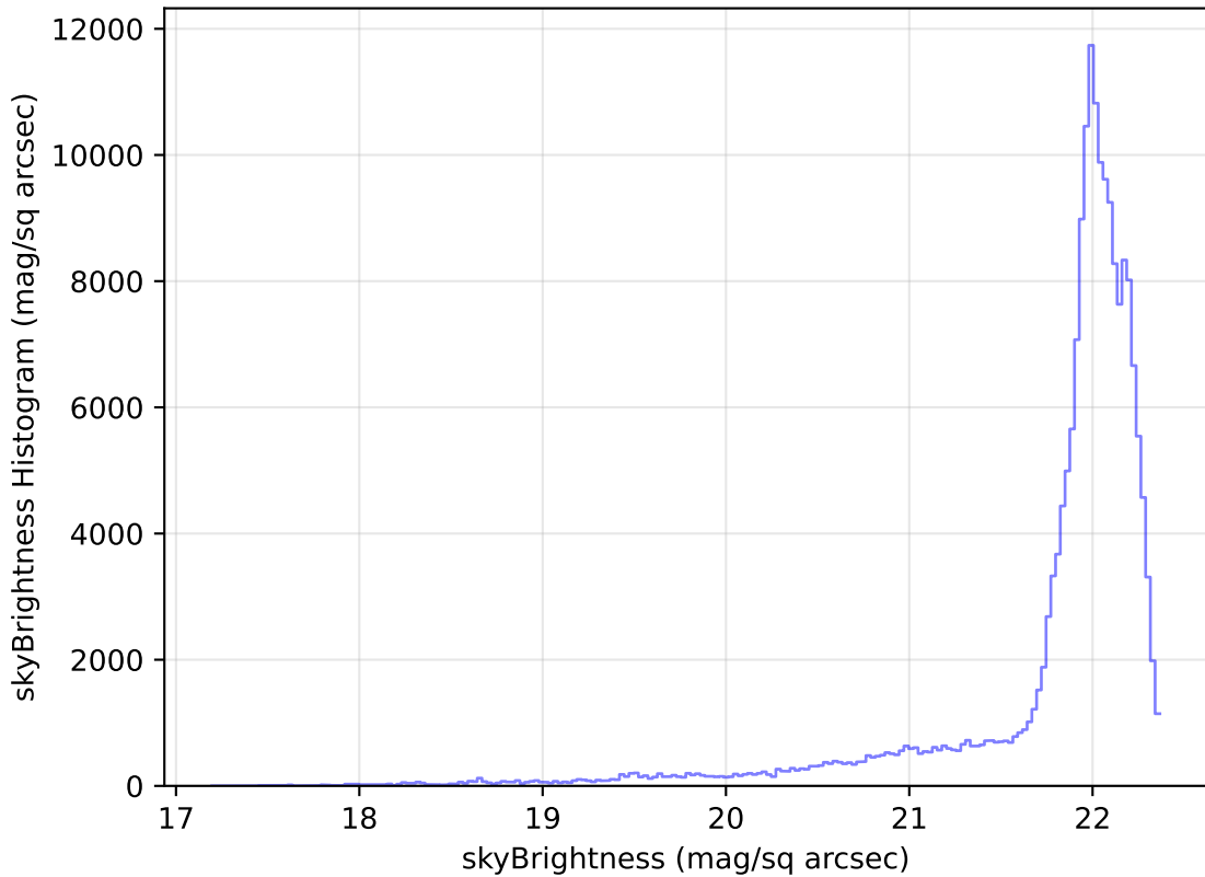
too_elab_r16_d3_ugrizy_v3.4_10yrs WFD g band: skyBrightness Histogram
