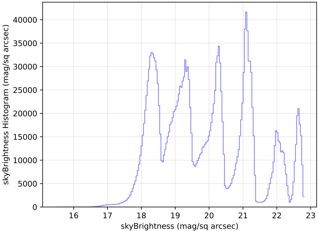
too_elab_r16_d3_ugrizy_v3.4_10yrs WFD all bands: skyBrightness Histogram
