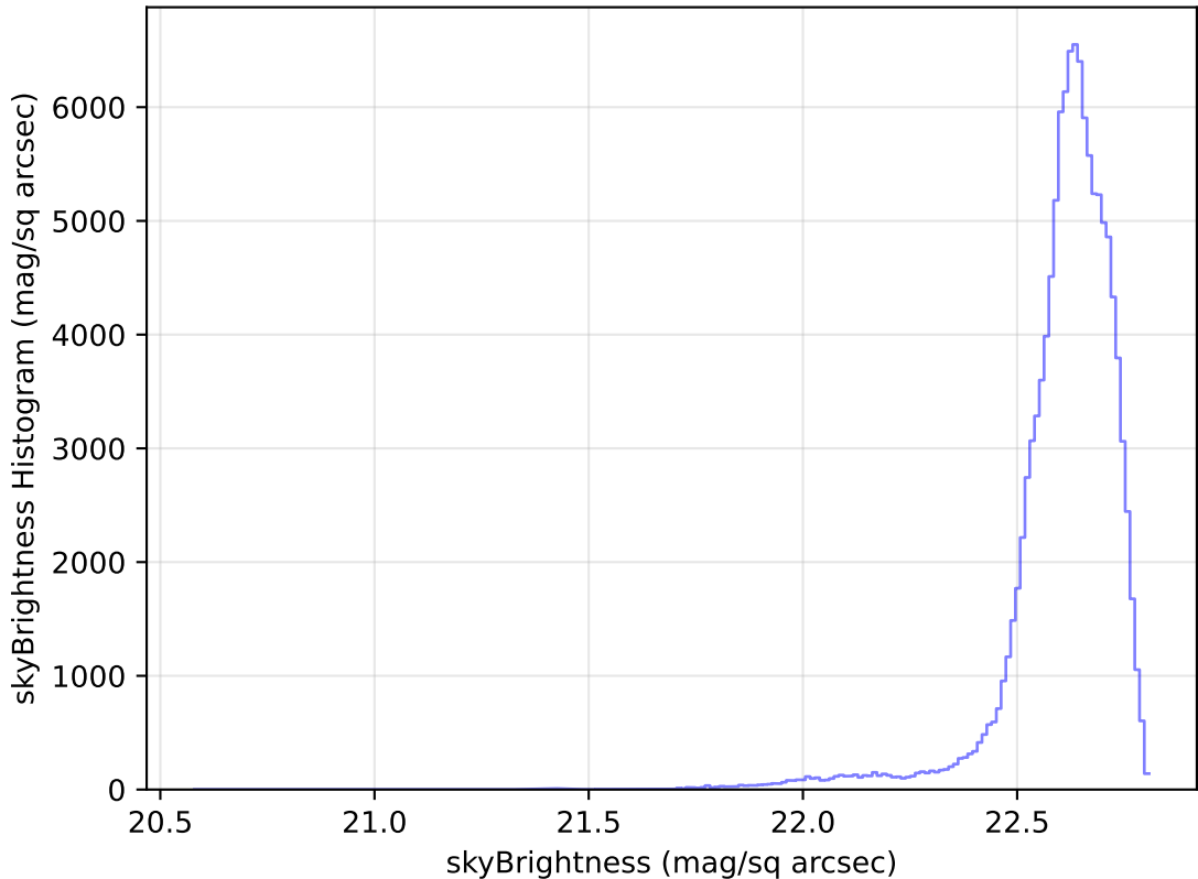
too_elab_r16_d3_ugrizy_v3.4_10yrs All sky u band: skyBrightness Histogram
