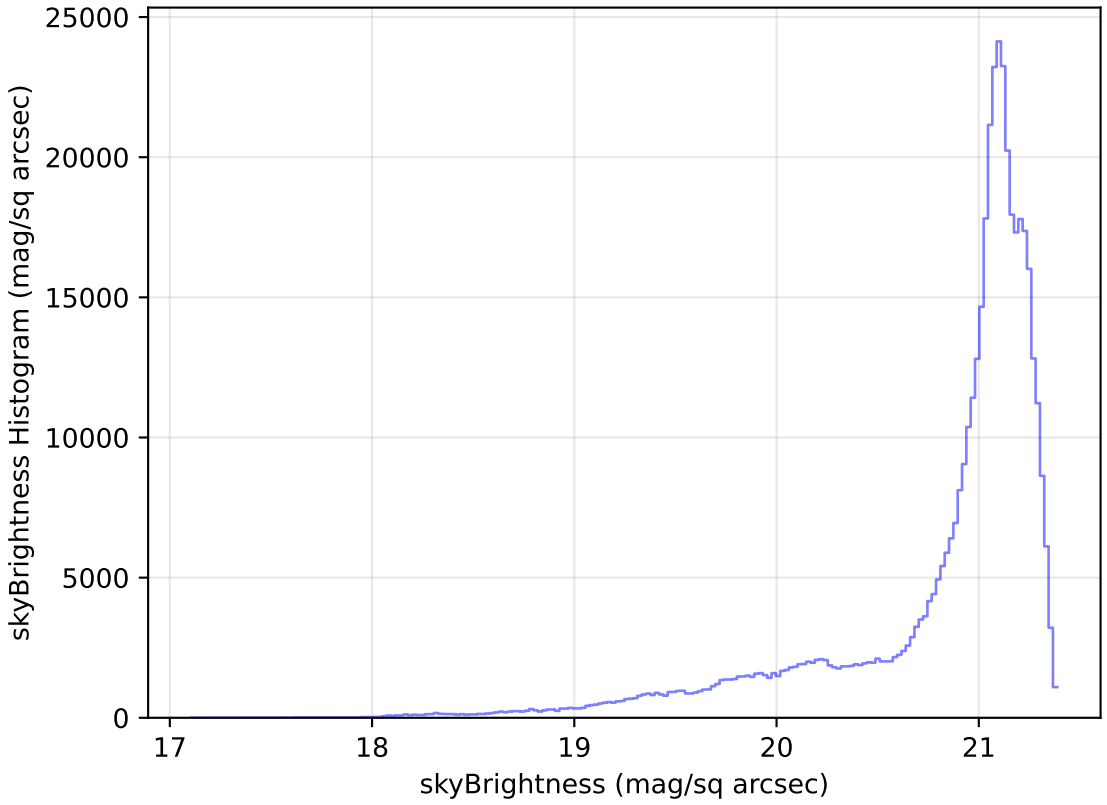
too_elab_r16_d3_ugrizy_v3.4_10yrs All sky r band: skyBrightness Histogram
