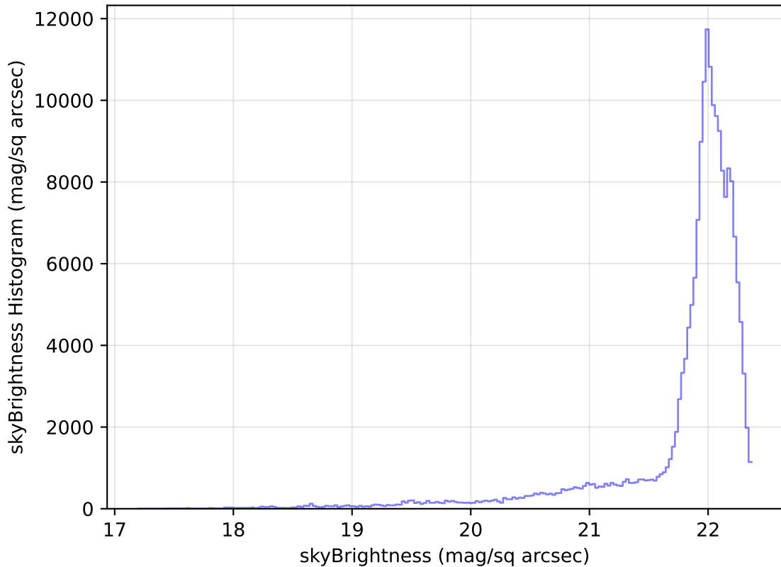
too_elab_r16_d3_ugrizy_v3.4_10yrs All sky g band: skyBrightness Histogram
