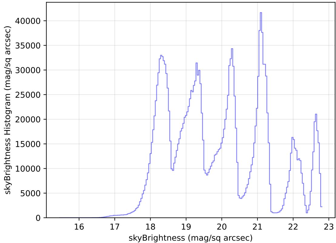
too_elab_r16_d3_ugrizy_v3.4_10yrs All sky all bands: skyBrightness Histogram
