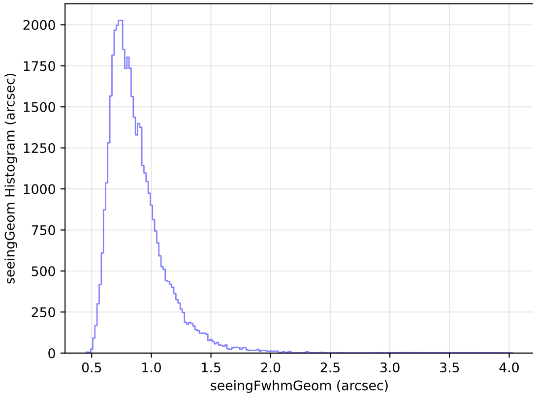
too_elab_r16_d3_ugrizy_v3.4_10yrs Yr 1 z band: seeingGeom Histogram
