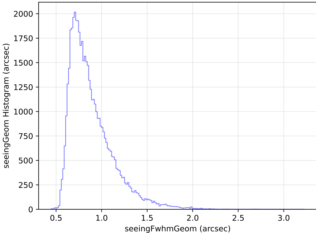
too_elab_r16_d3_ugrizy_v3.4_10yrs Yr 1 r band: seeingGeom Histogram
