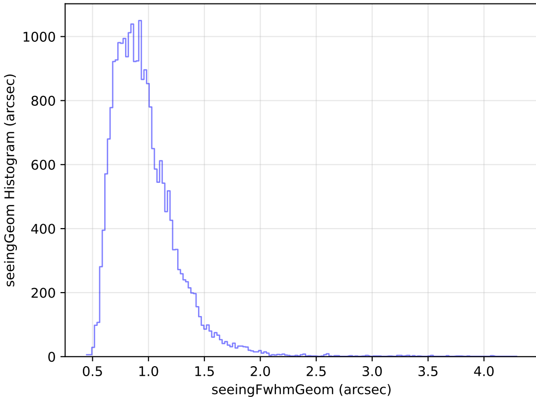
too_elab_r16_d3_ugrizy_v3.4_10yrs Yr 1 g band: seeingGeom Histogram
