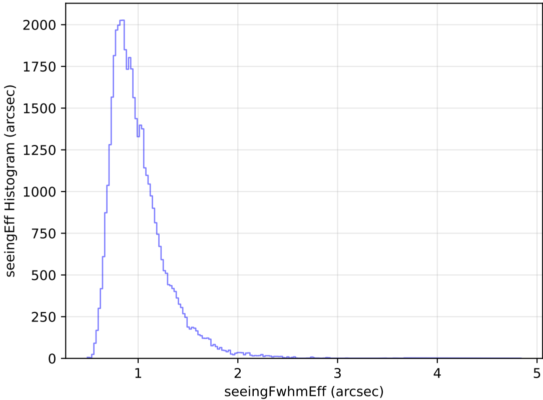
too_elab_r16_d3_ugrizy_v3.4_10yrs Yr 1 z band: seeingEff Histogram
