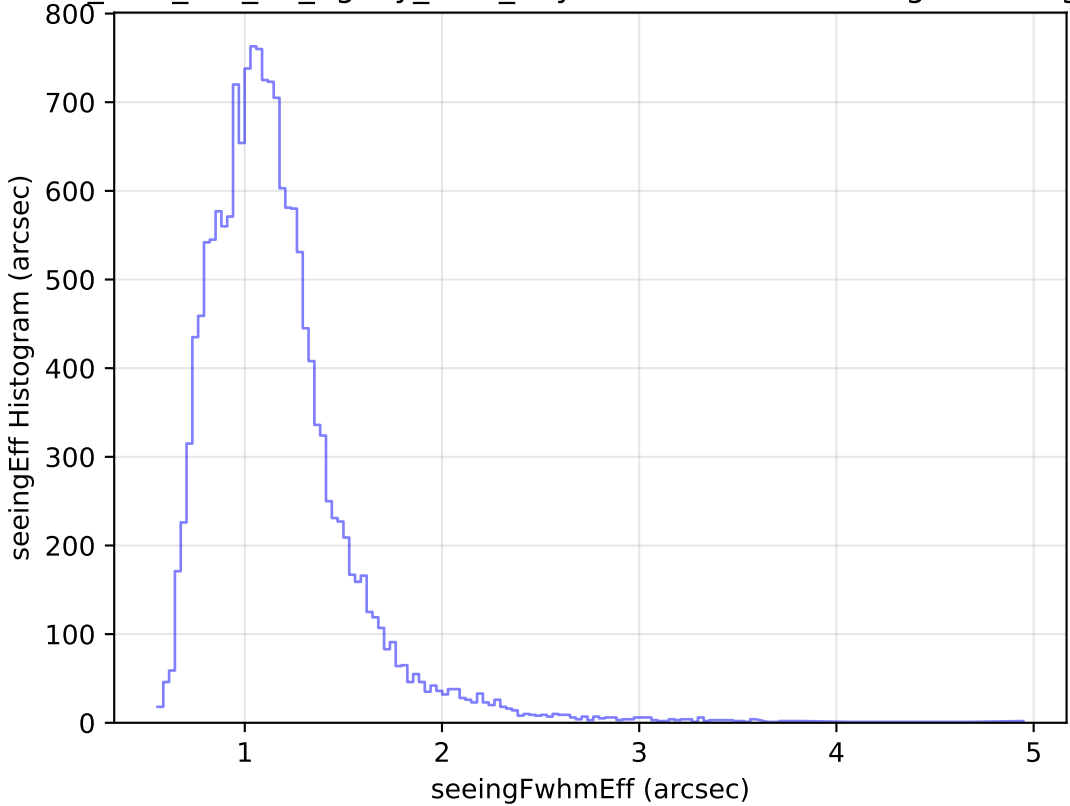
too_elab_r16_d3_ugrizy_v3.4_10yrs Yr 1 u band: seeingEff Histogram
