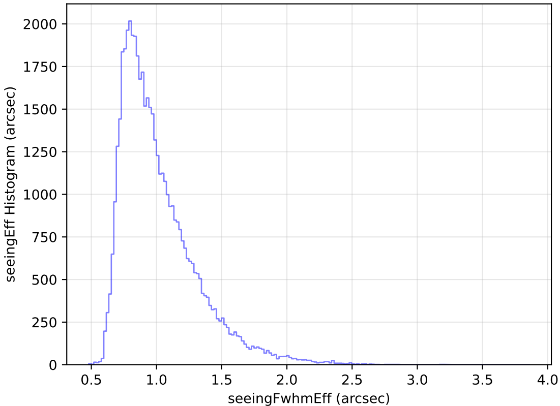
too_elab_r16_d3_ugrizy_v3.4_10yrs Yr 1 r band: seeingEff Histogram
