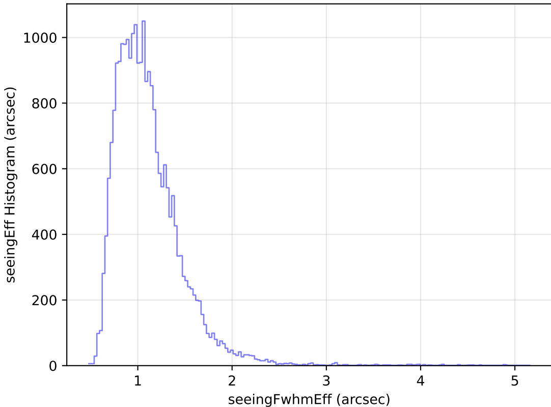
too_elab_r16_d3_ugrizy_v3.4_10yrs Yr 1 g band: seeingEff Histogram
