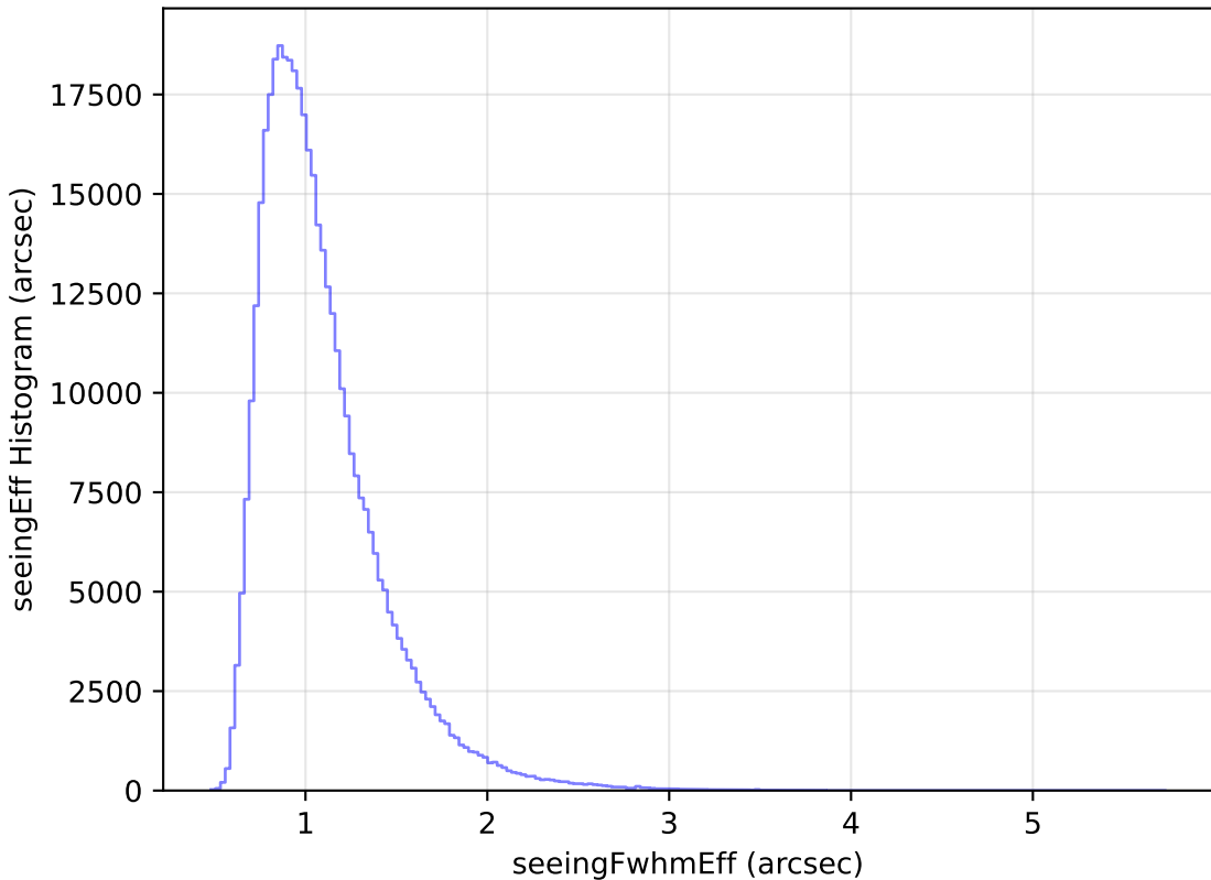
too_elab_r16_d3_ugrizy_v3.4_10yrs WFD z band: seeingEff Histogram
