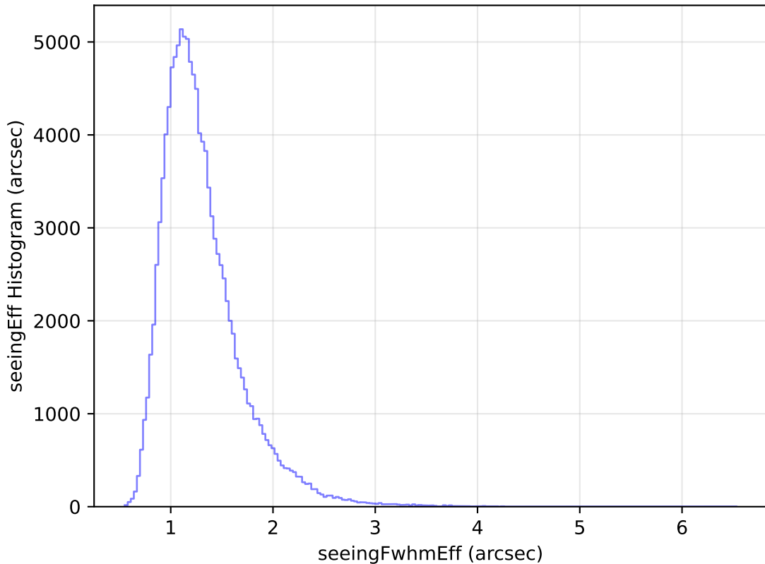
too_elab_r16_d3_ugrizy_v3.4_10yrs WFD u band: seeingEff Histogram
