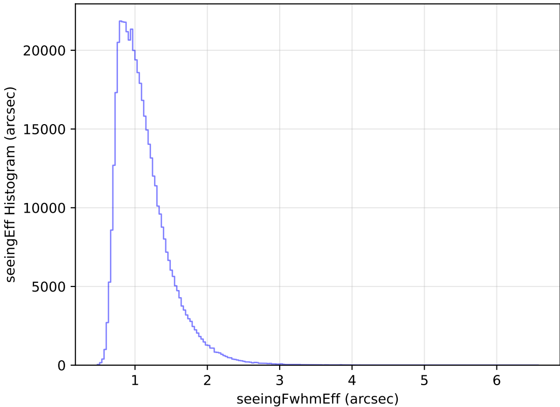
too_elab_r16_d3_ugrizy_v3.4_10yrs WFD r band: seeingEff Histogram
