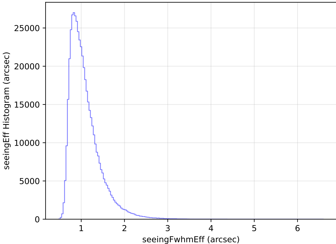
too_elab_r16_d3_ugrizy_v3.4_10yrs WFD i band: seeingEff Histogram
