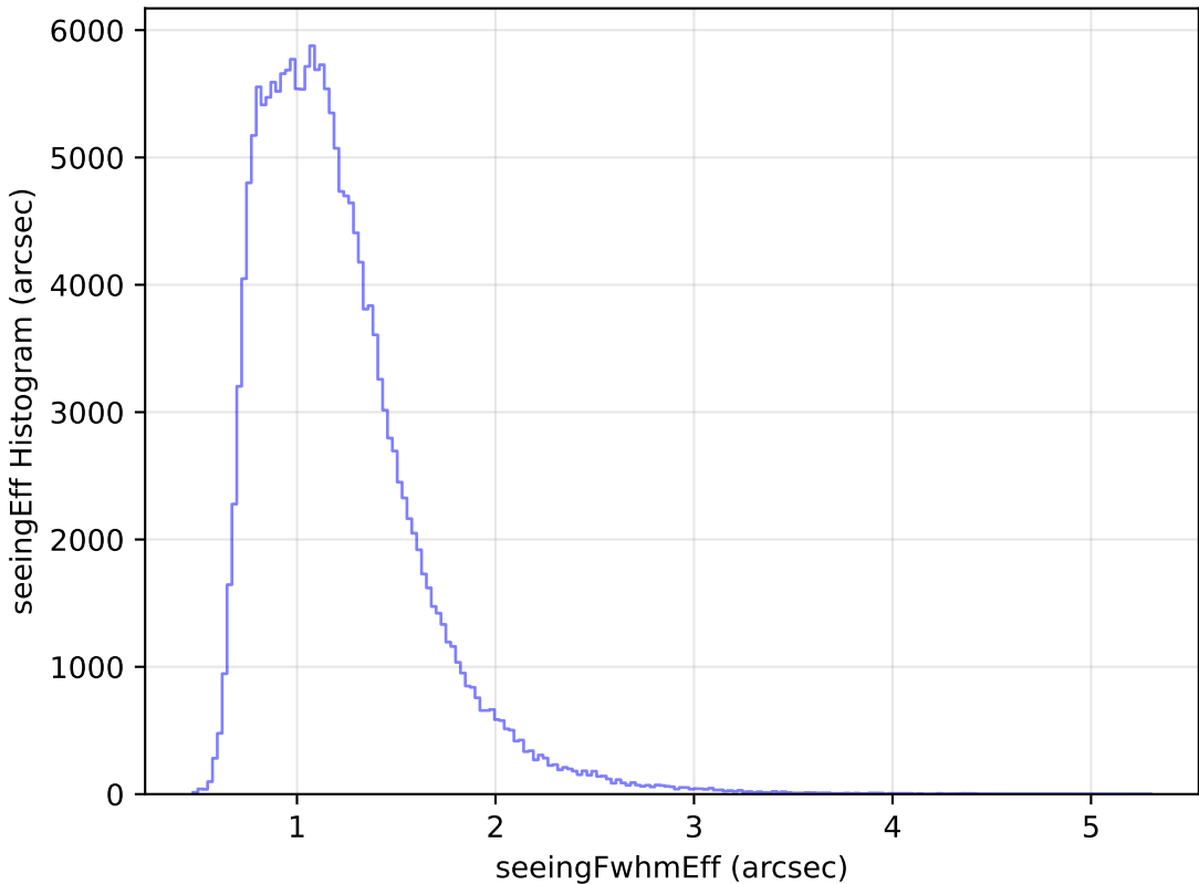
too_elab_r16_d3_ugrizy_v3.4_10yrs WFD g band: seeingEff Histogram
