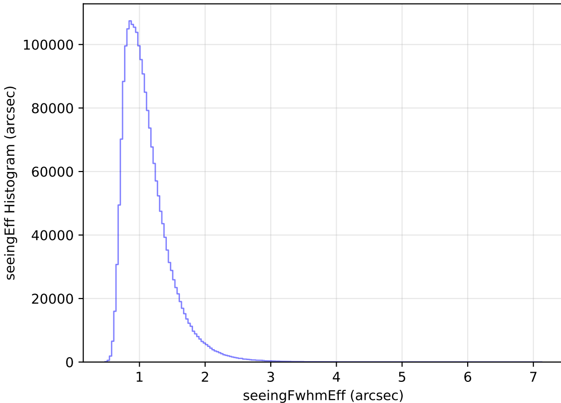
too_elab_r16_d3_ugrizy_v3.4_10yrs WFD all bands: seeingEff Histogram
