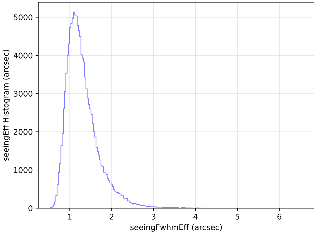
too_elab_r16_d3_ugrizy_v3.4_10yrs All sky u band: seeingEff Histogram
