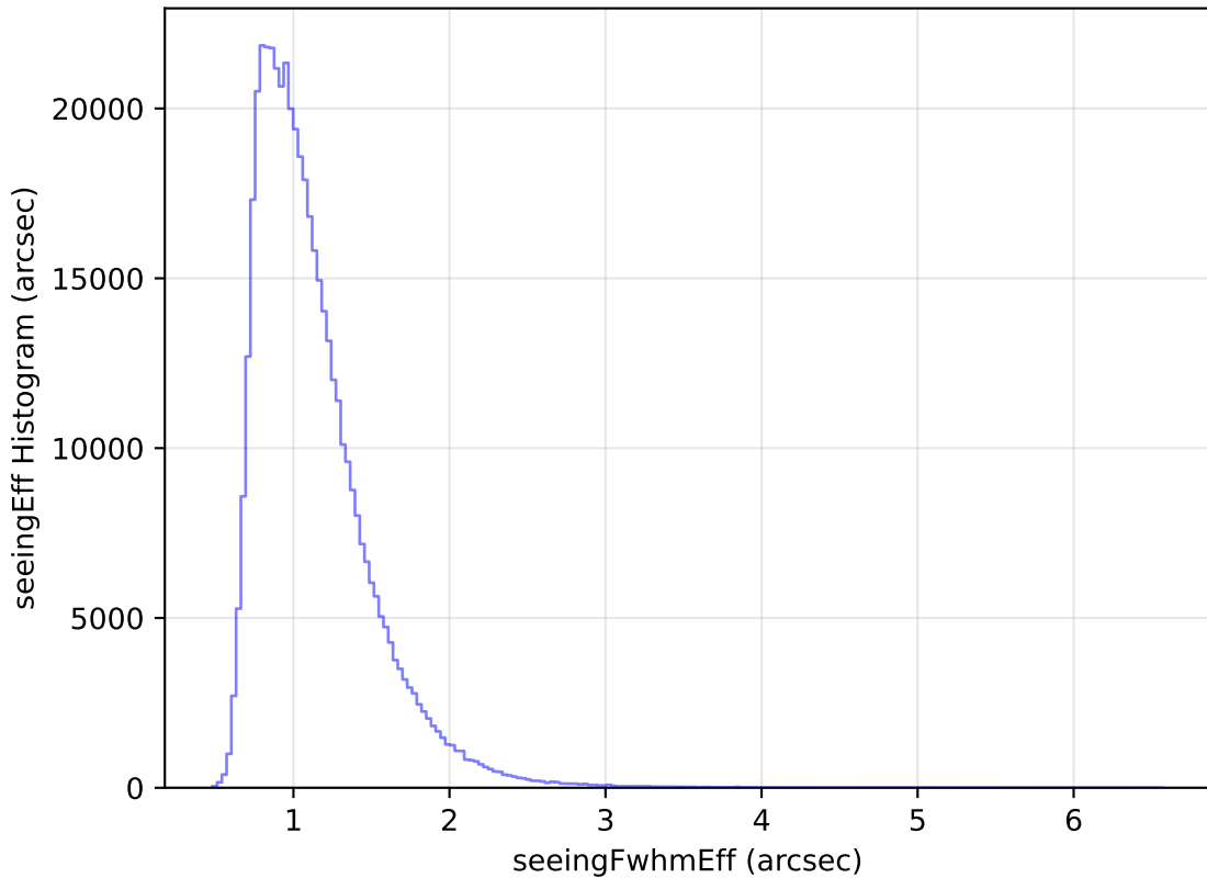
too_elab_r16_d3_ugrizy_v3.4_10yrs All sky r band: seeingEff Histogram
