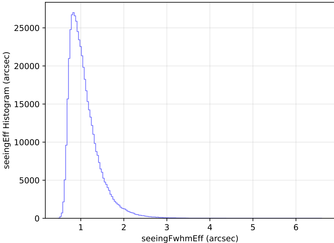
too_elab_r16_d3_ugrizy_v3.4_10yrs All sky i band: seeingEff Histogram
