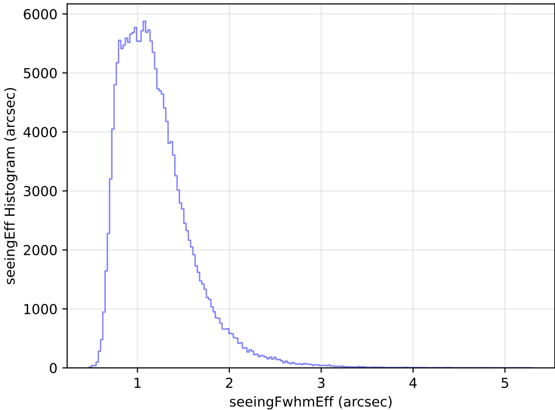
too_elab_r16_d3_ugrizy_v3.4_10yrs All sky g band: seeingEff Histogram
