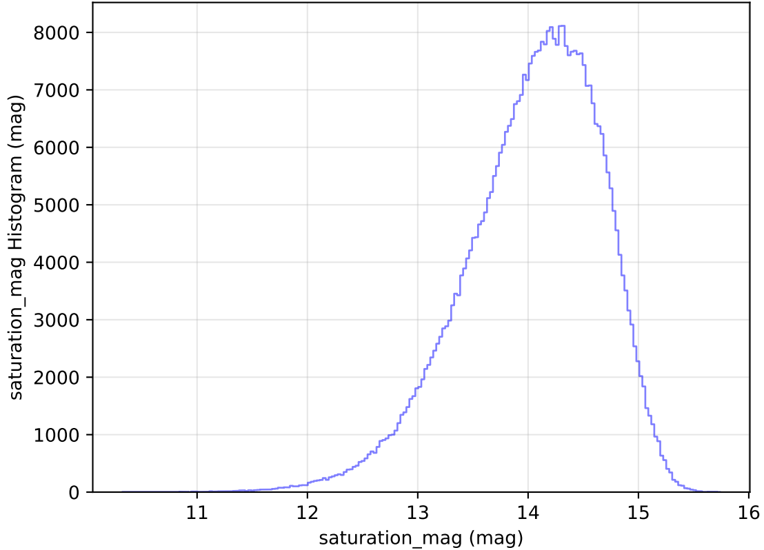
too_elab_r16_d3_ugrizy_v3.4_10yrs WFD z band: saturation_mag Histogram
