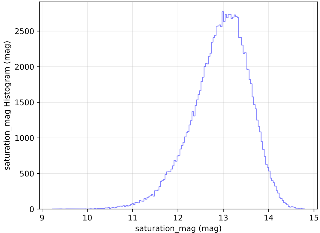
too_elab_r16_d3_ugrizy_v3.4_10yrs WFD u band: saturation_mag Histogram
