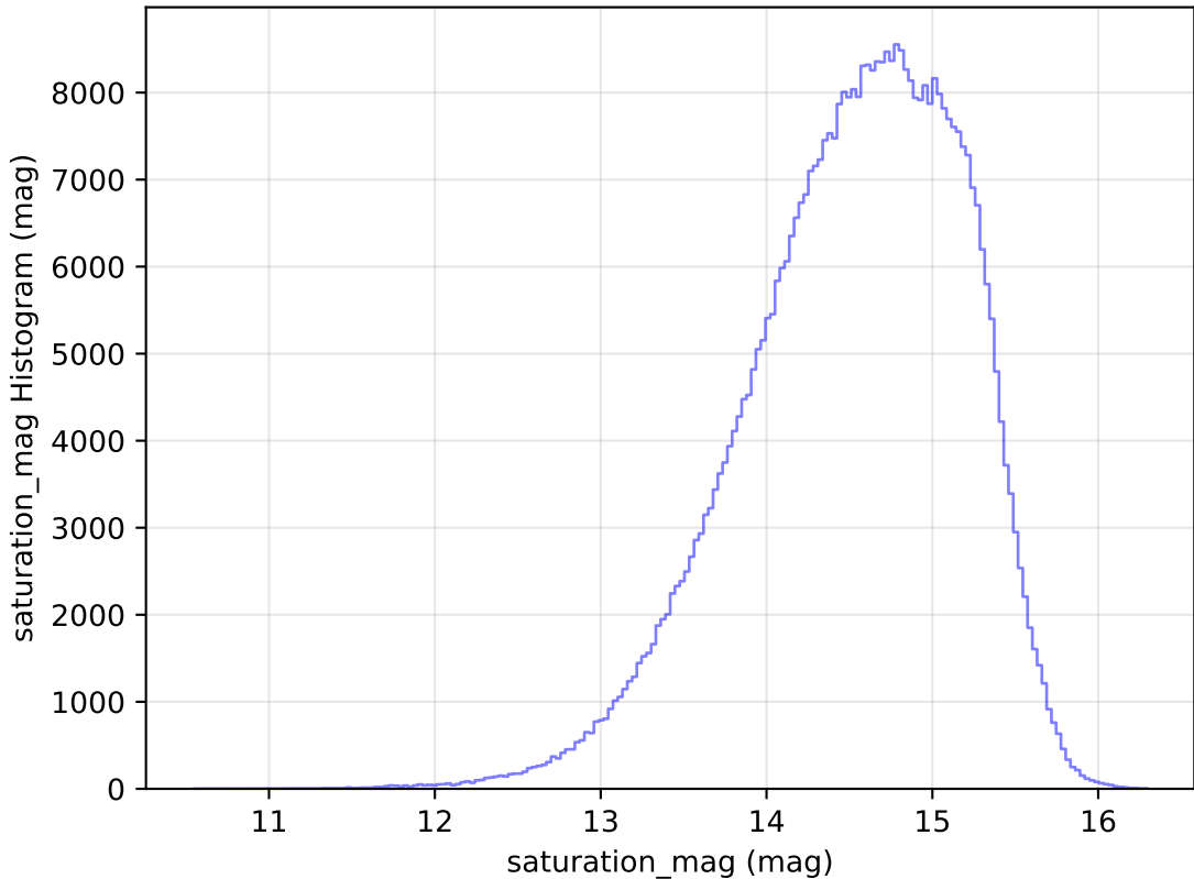
too_elab_r16_d3_ugrizy_v3.4_10yrs WFD r band: saturation_mag Histogram
