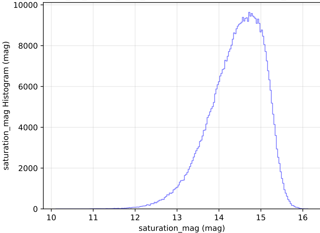
too_elab_r16_d3_ugrizy_v3.4_10yrs WFD i band: saturation_mag Histogram
