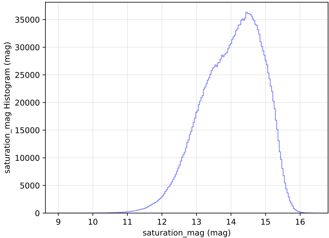
too_elab_r16_d3_ugrizy_v3.4_10yrs WFD all bands: saturation_mag Histogram
