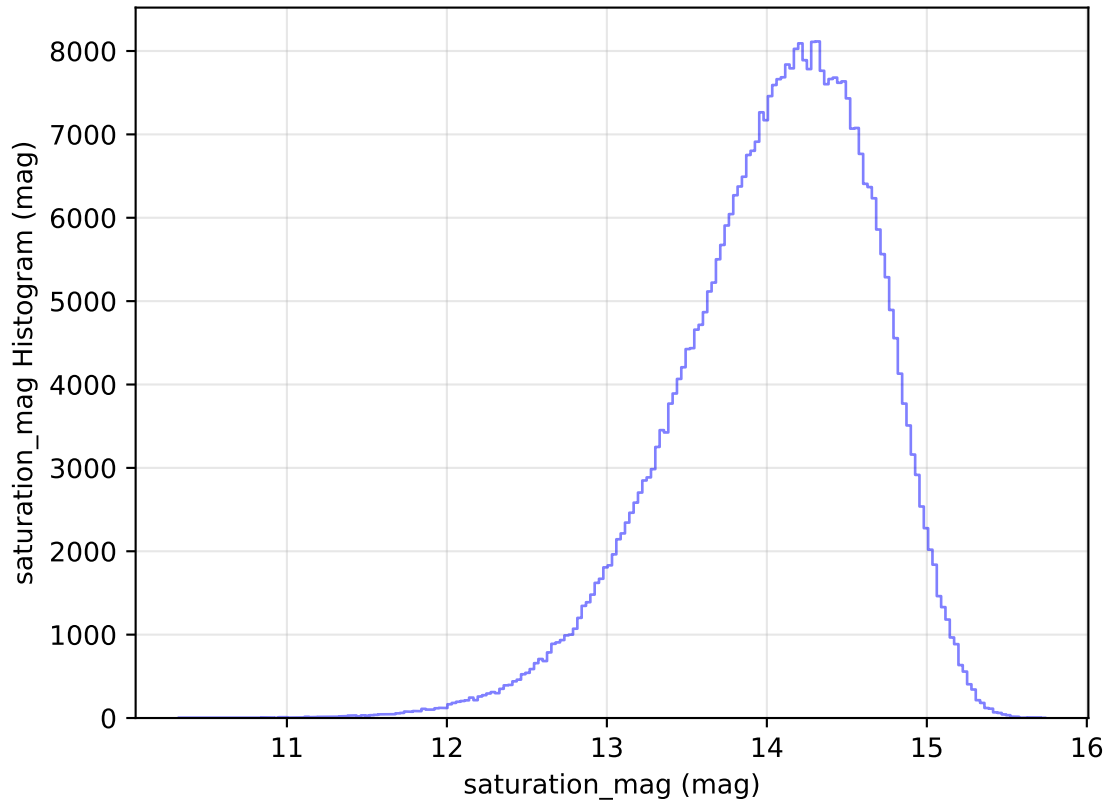
too_elab_r16_d3_ugrizy_v3.4_10yrs All sky z band: saturation_mag Histogram
