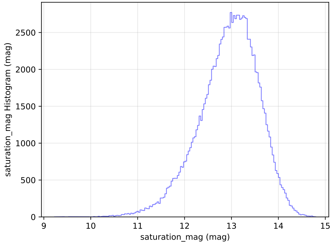
too_elab_r16_d3_ugrizy_v3.4_10yrs All sky u band: saturation_mag Histogram
