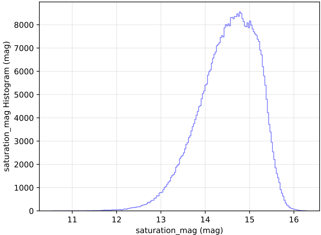
too_elab_r16_d3_ugrizy_v3.4_10yrs All sky r band: saturation_mag Histogram
