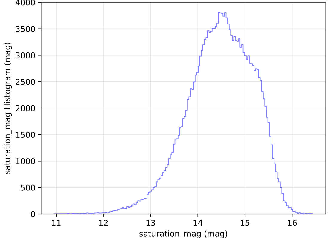
too_elab_r16_d3_ugrizy_v3.4_10yrs All sky g band: saturation_mag Histogram
