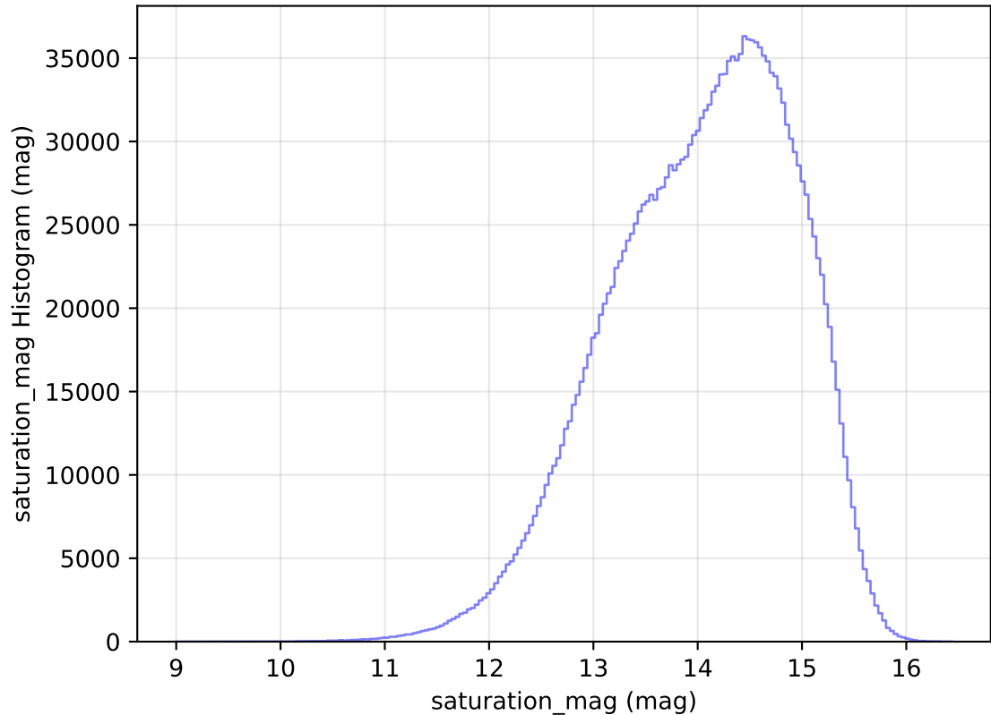
too_elab_r16_d3_ugrizy_v3.4_10yrs All sky all bands: saturation_mag Histogram
