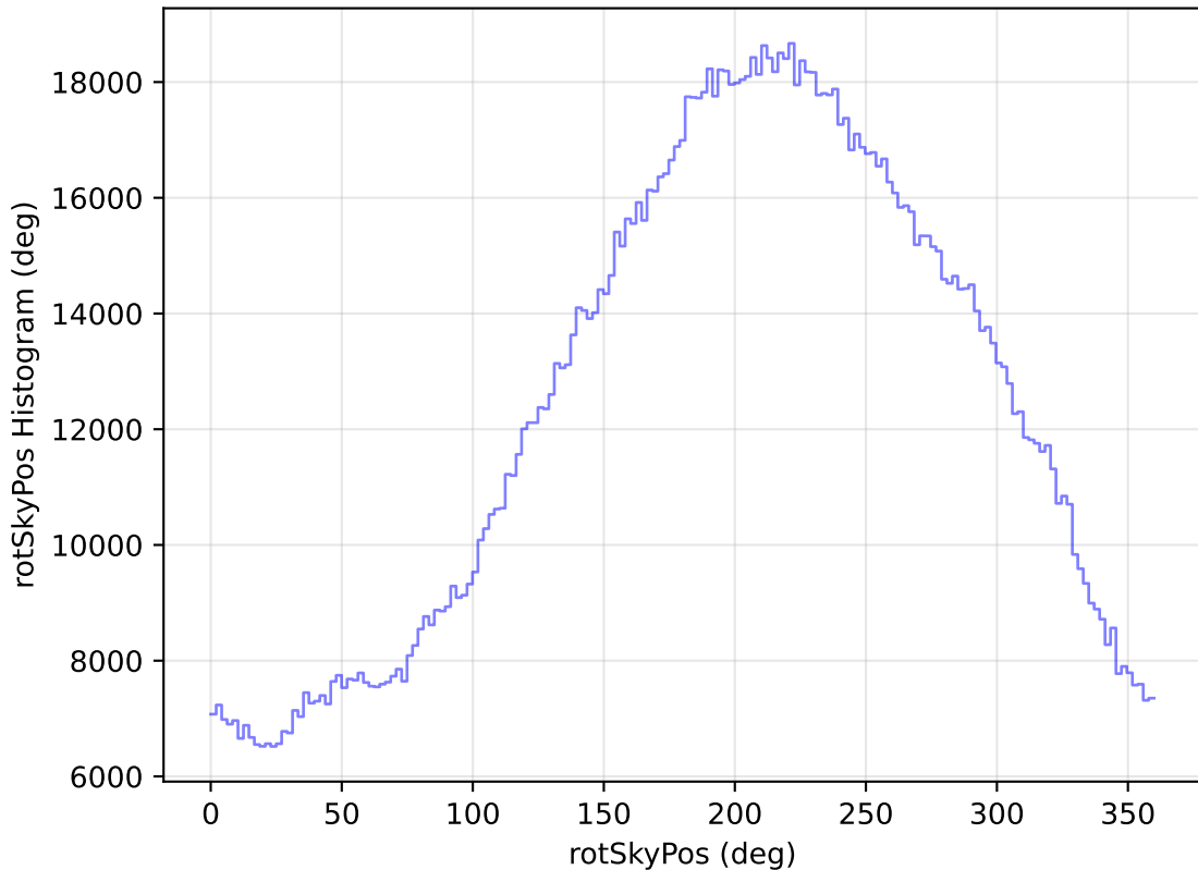
too_elab_r16_d3_ugrizy_v3.4_10yrs WFD all bands: rotSkyPos Histogram
