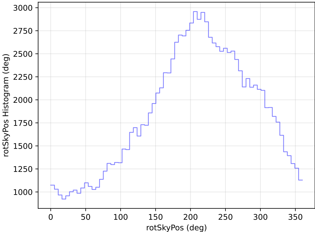
too_elab_r16_d3_ugrizy_v3.4_10yrs All sky u band: rotSkyPos Histogram
