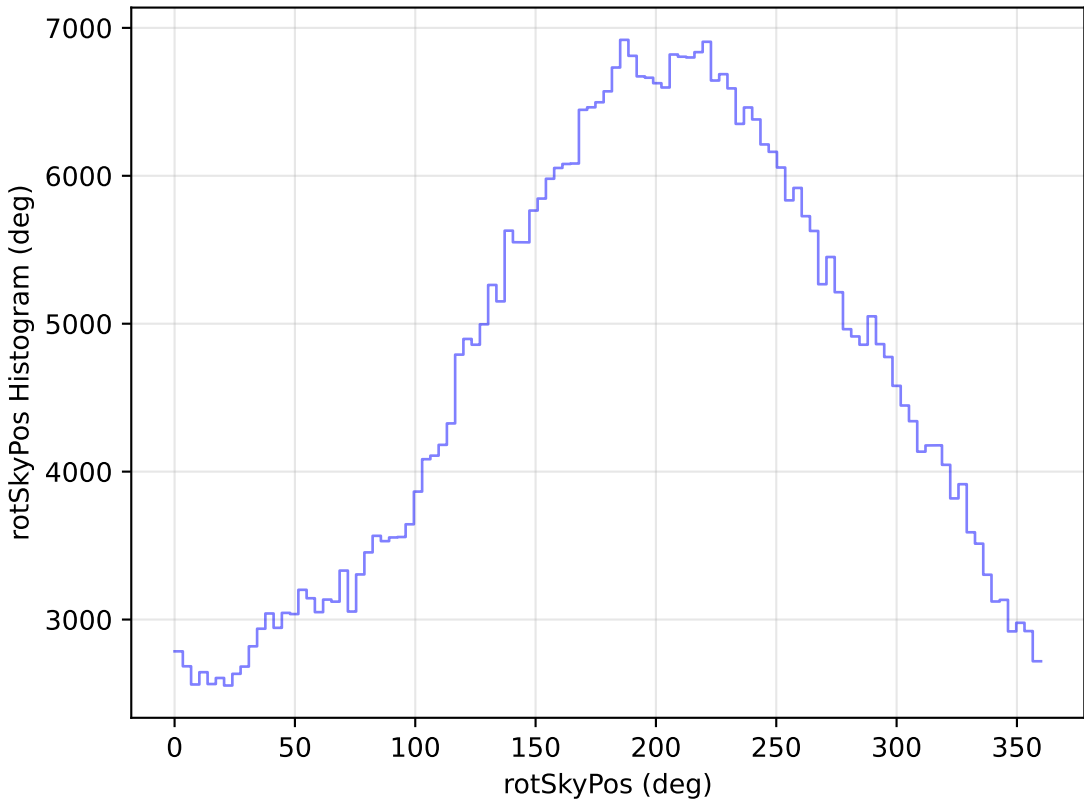
too_elab_r16_d3_ugrizy_v3.4_10yrs All sky r band: rotSkyPos Histogram
