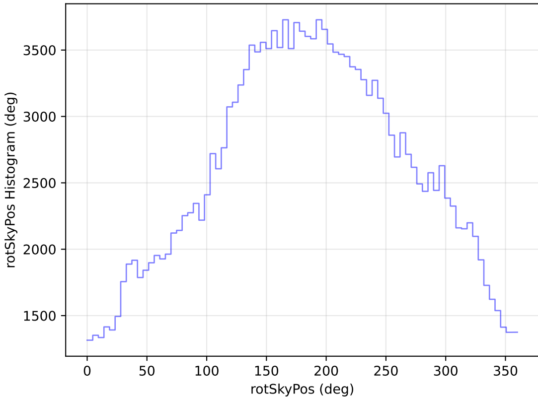
too_elab_r16_d3_ugrizy_v3.4_10yrs All sky g band: rotSkyPos Histogram
