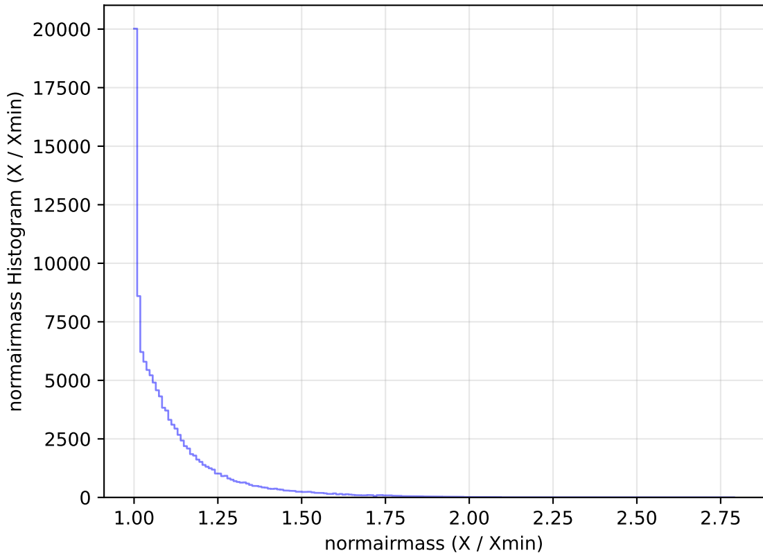
too_elab_r16_d3_ugrizy_v3.4_10yrs WFD u band: normairmass Histogram
