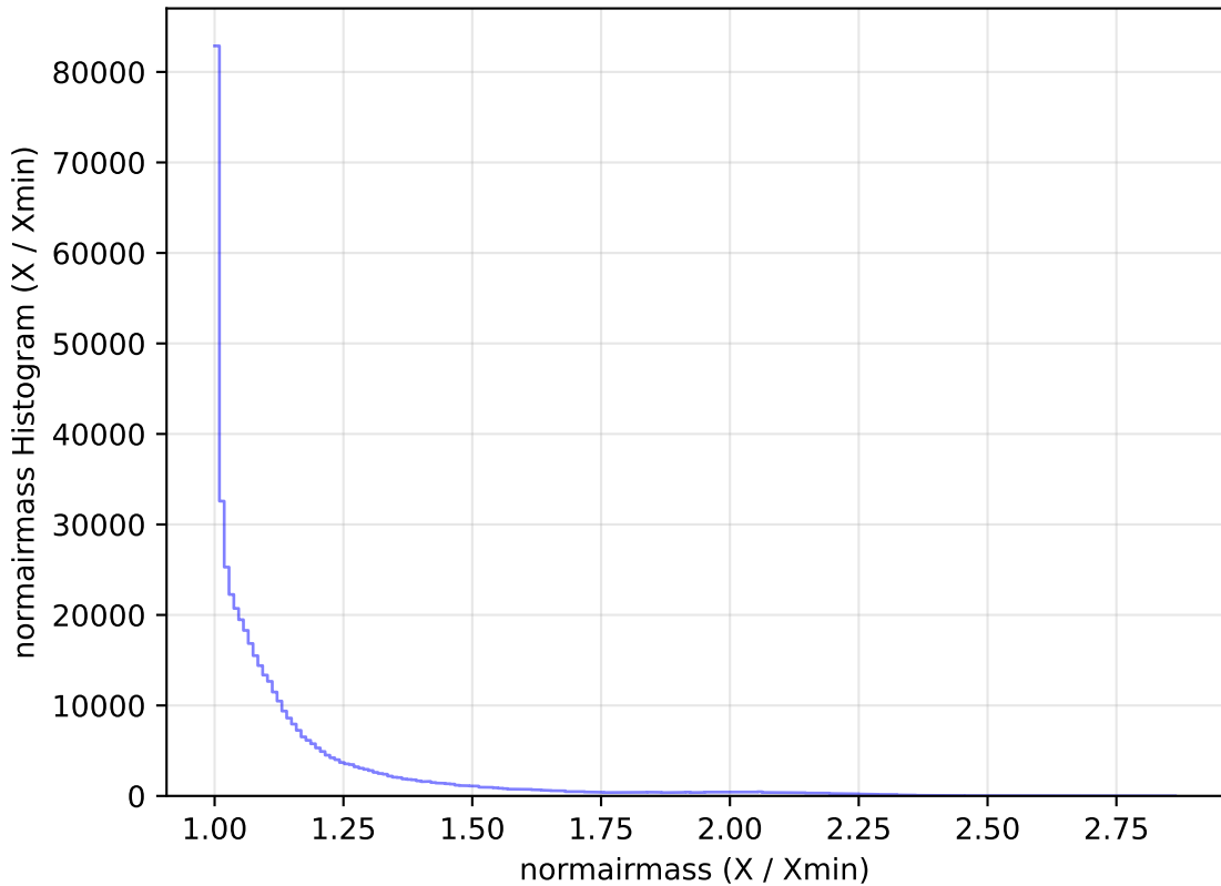
too_elab_r16_d3_ugrizy_v3.4_10yrs WFD r band: normairmass Histogram
