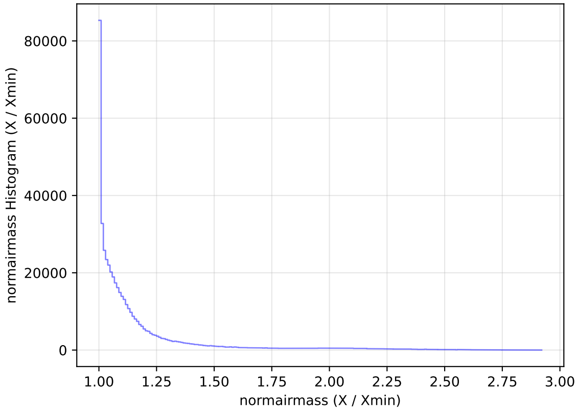
too_elab_r16_d3_ugrizy_v3.4_10yrs WFD i band: normairmass Histogram
