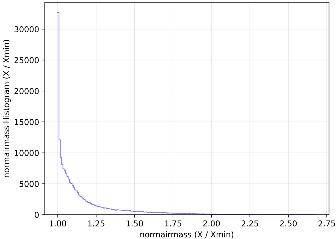
too_elab_r16_d3_ugrizy_v3.4_10yrs WFD g band: normairmass Histogram
