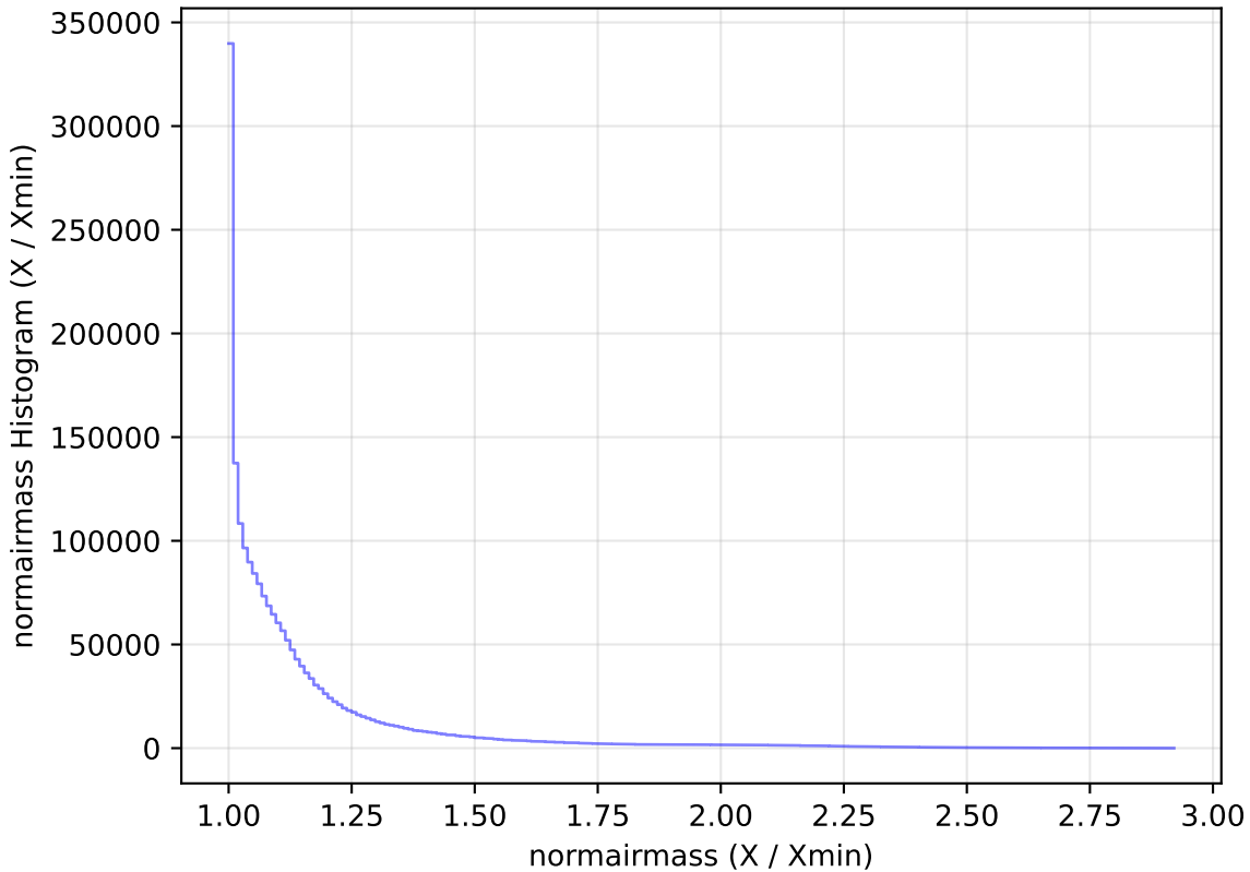
too_elab_r16_d3_ugrizy_v3.4_10yrs WFD all bands: normairmass Histogram
