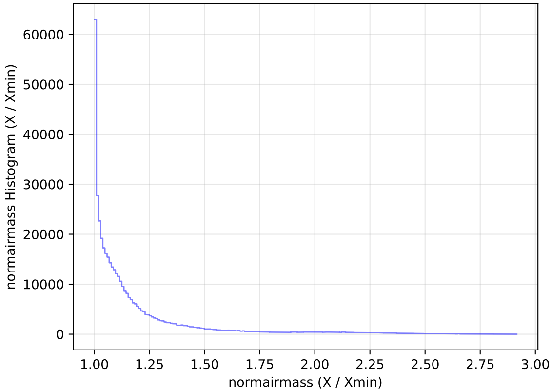
too_elab_r16_d3_ugrizy_v3.4_10yrs All sky z band: normairmass Histogram
