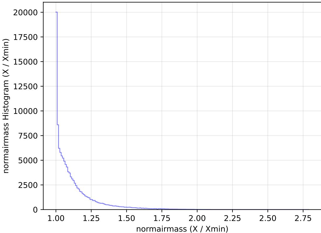
too_elab_r16_d3_ugrizy_v3.4_10yrs All sky u band: normairmass Histogram
