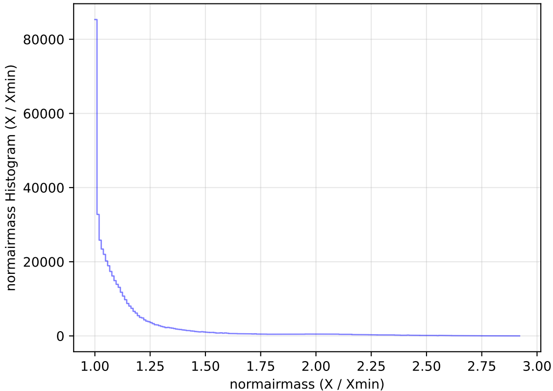
too_elab_r16_d3_ugrizy_v3.4_10yrs All sky i band: normairmass Histogram
