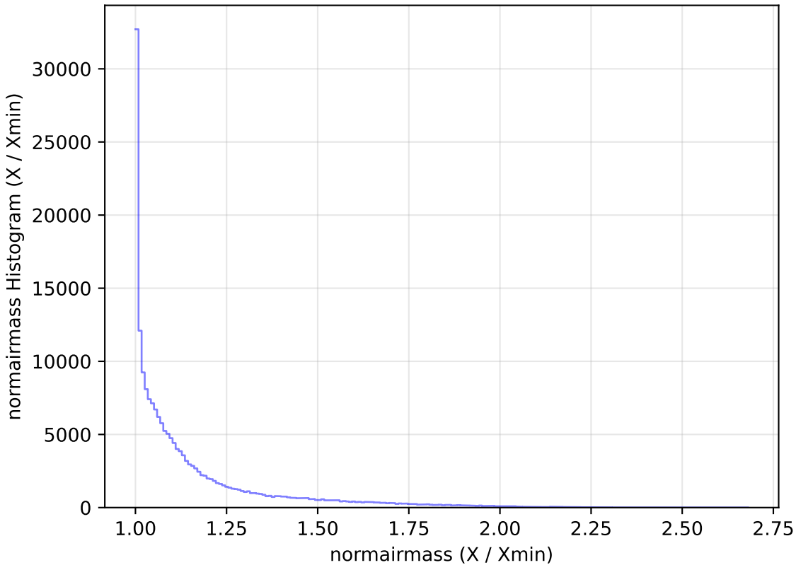
too_elab_r16_d3_ugrizy_v3.4_10yrs All sky g band: normairmass Histogram
