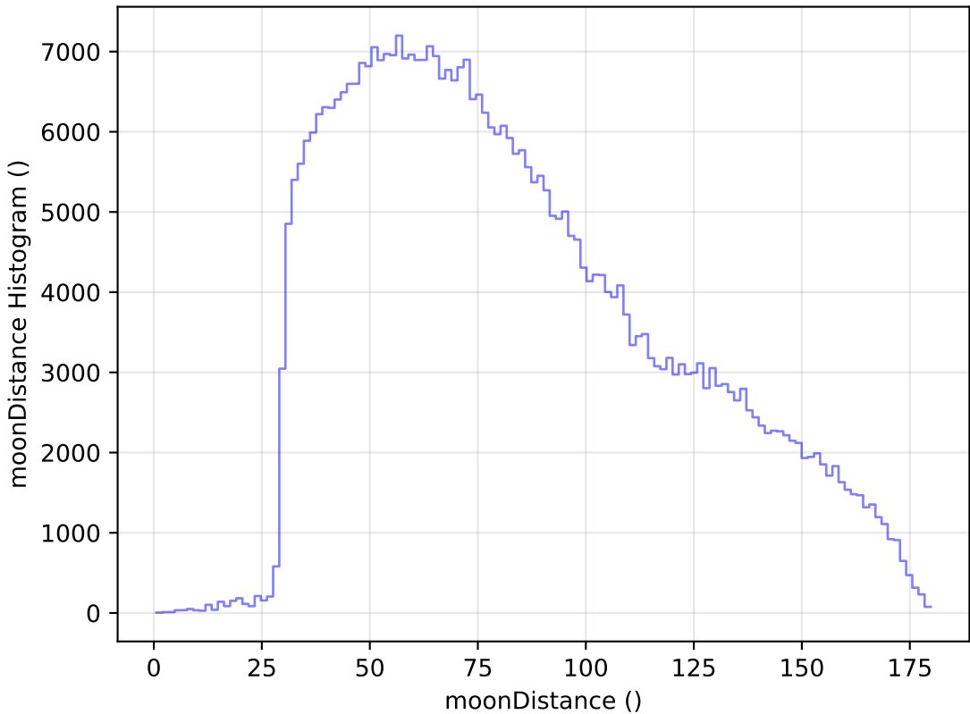
too_elab_r16_d3_ugrizy_v3.4_10yrs WFD z band: moonDistance Histogram
