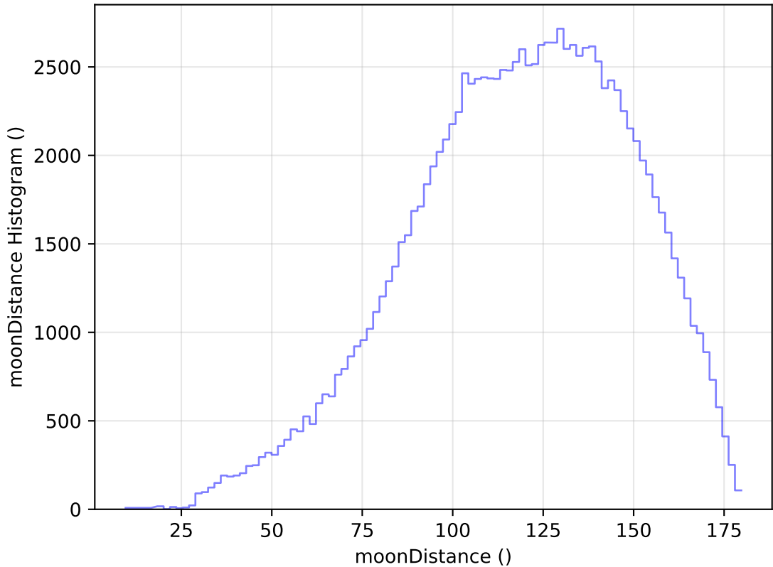
too_elab_r16_d3_ugrizy_v3.4_10yrs WFD u band: moonDistance Histogram
