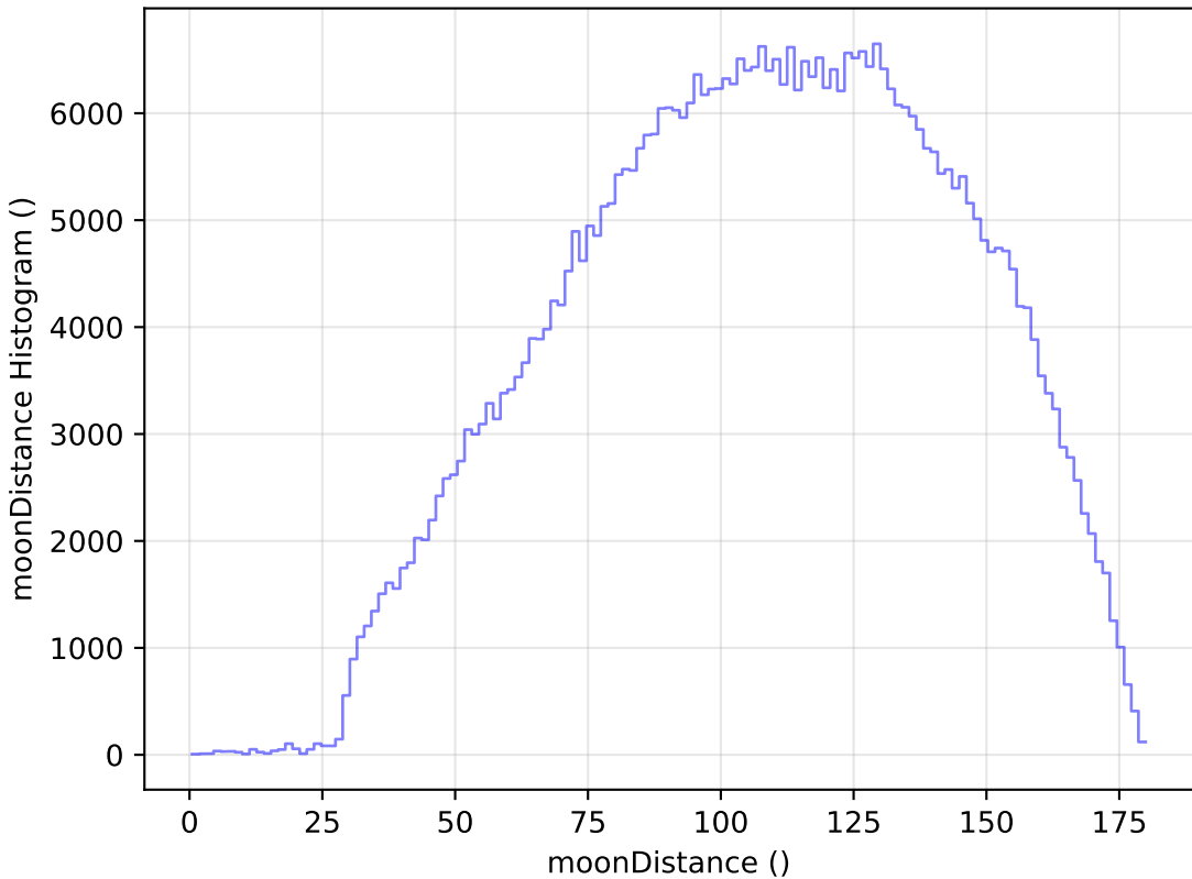
too_elab_r16_d3_ugrizy_v3.4_10yrs WFD r band: moonDistance Histogram
