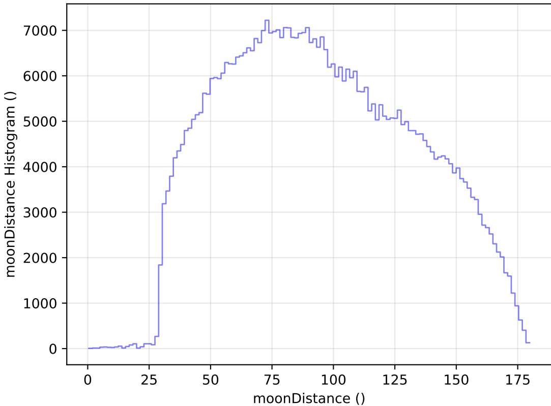
too_elab_r16_d3_ugrizy_v3.4_10yrs WFD i band: moonDistance Histogram
